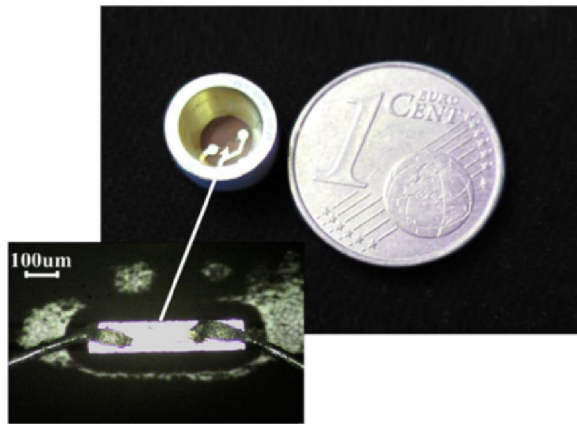
Figure 5: A Single Propulsion-Less Micro-Drift (Xianti & Associates, 2010: 230)
