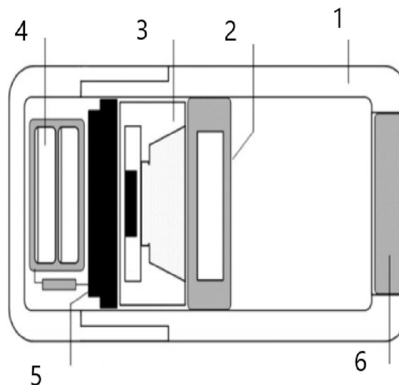
Figure 1: Remote-Controlled Capsule's Structure (Xianti & Associates, 2010: 228)
