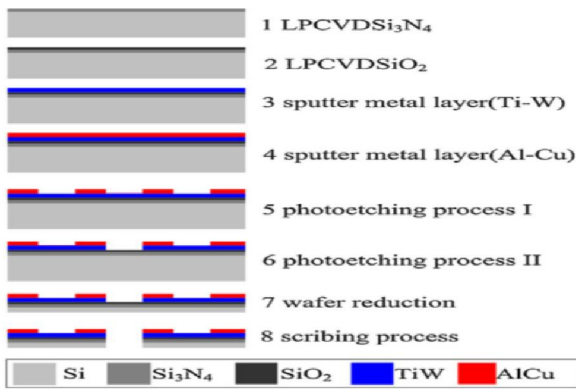
Figure 4: Microfiber Ignition Fabrication Process (Xianti & Associates, 2010: 229)
