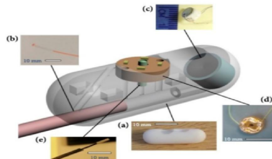
Figure 18: An Initial Capsule For Targeted Ultrasound-Mediated Drug Delivery (Cortegoso Valdivia & Associates, 2021: 4), Wherein: A) Body Of capsule, B) Connection To Power Cables & Drug Delivery Channel, C) Ultrasound Probe, D) Light Source & E) Miniature Camera
