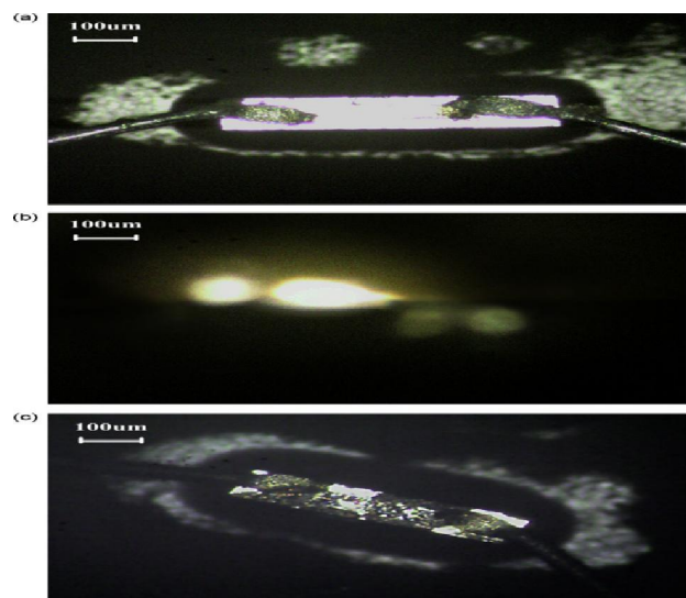
Figure 6: Images Of Micro-Igniters Before, During & After Combustion. (A), Non-Propulsion Micro-Drift (B) During Combustion & Ignition (C) After Successful Combustion (Xianti & Associates, 2010: 230)
