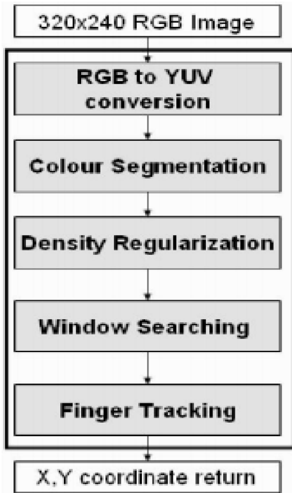
Figure 5: YUV Color Space Finger Tracking Flow (Courtesy Tsang et. Al. [39])
