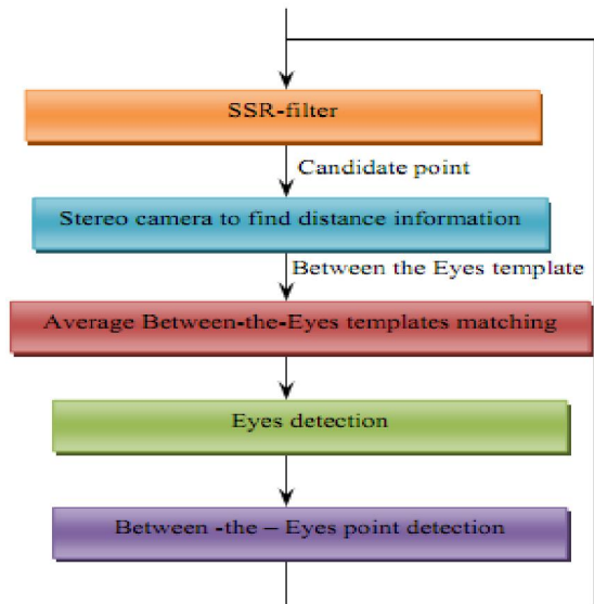
Figure 2: Flow Diagram Of Real Time Face Detection (Courtesy Sumathi et. Al. [8])
