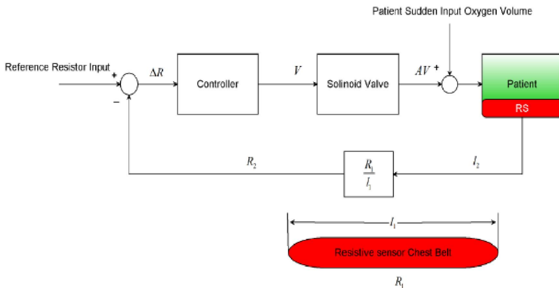
Figure 1 block diagram of the ventilator system
