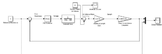
Figure 3 Simulink block diagram
