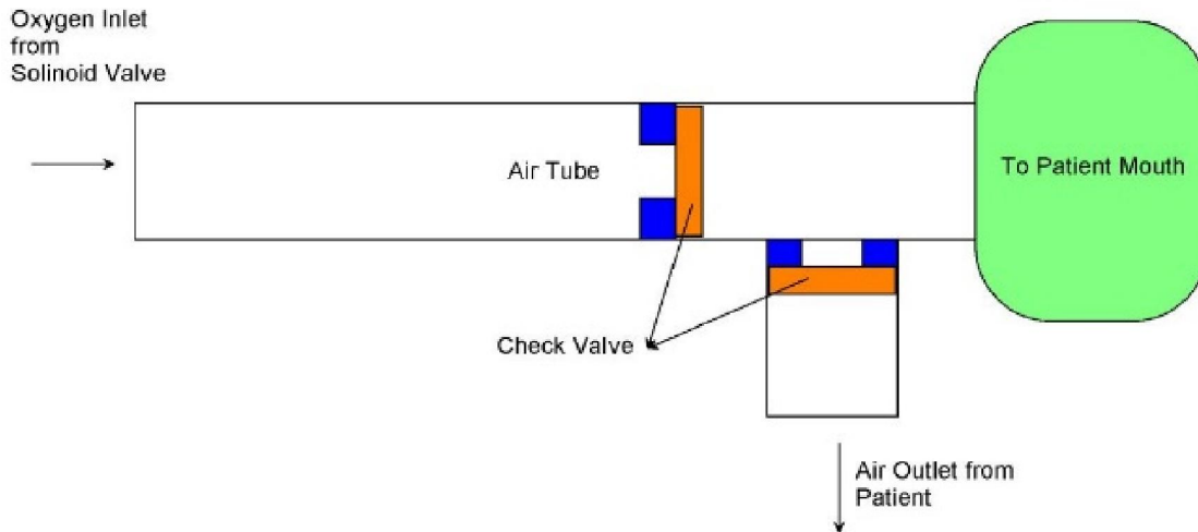
Figure 2 Ventilator air duct model
