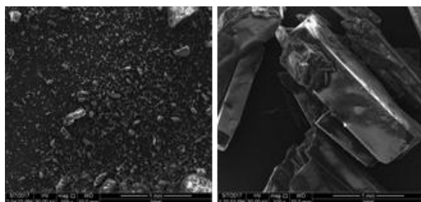
Figure (4): SEM micrographs of the gliclazide/malonic acid system (A) Physical mixture (B) co-precipitated mixture
