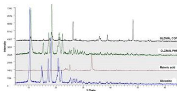
Figure (2): XRPD spectra of the gliclazide/malonic acid system
