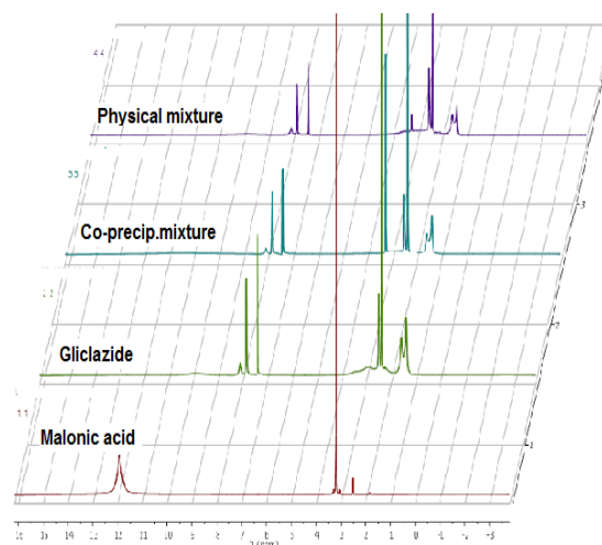
Figure (6): NMR spectra of gliclazide/malonic acid system
