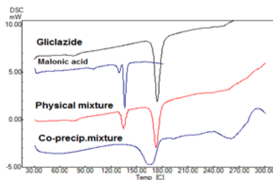
Figure (3): DSC traces of the gliclazide/ malonic acid system (sample weight 4-6 mg, scan rate 10^\circ\text{C}/\text{min} )
