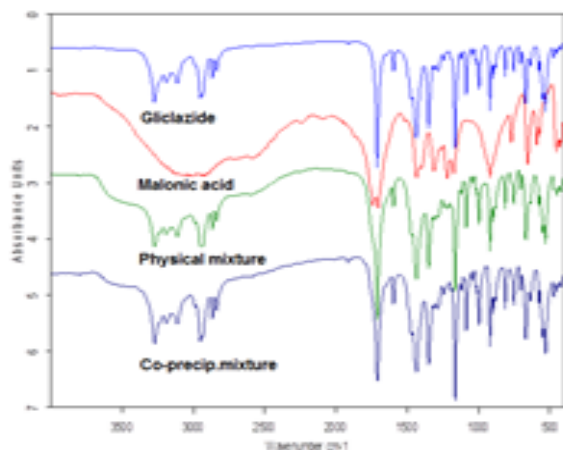
Figure (5): IR-spectra of gliclazide/malonic acid system
